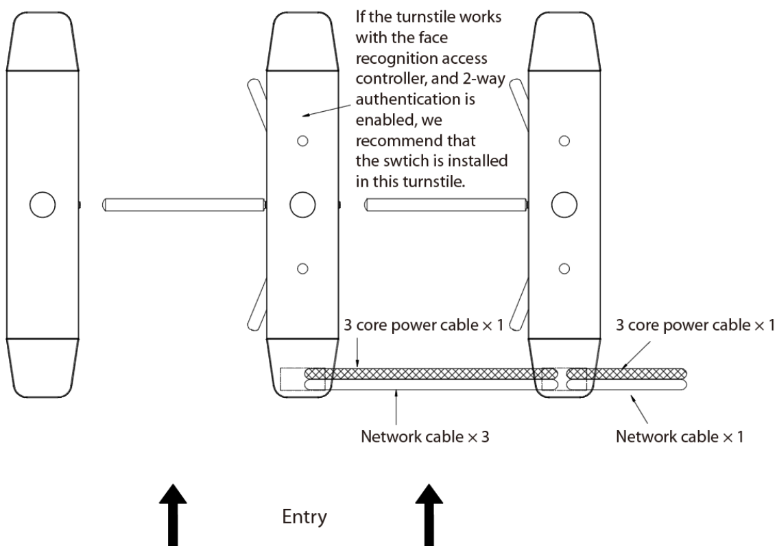
Figure 2-5 Wiring diagram
