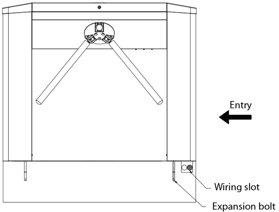
Figure 2-4 Wiring slot
