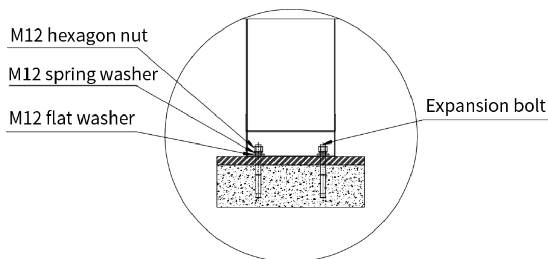
Figure 2-6 Secure turnstiles
